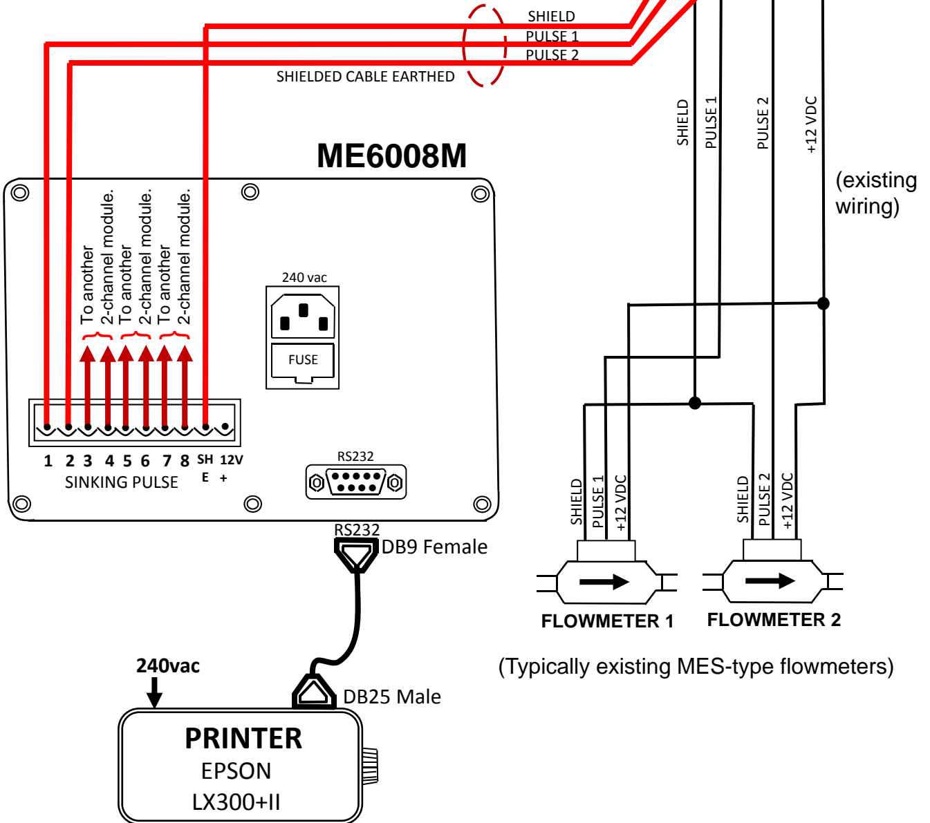
Wiring between ME2008 module and ME6008M
