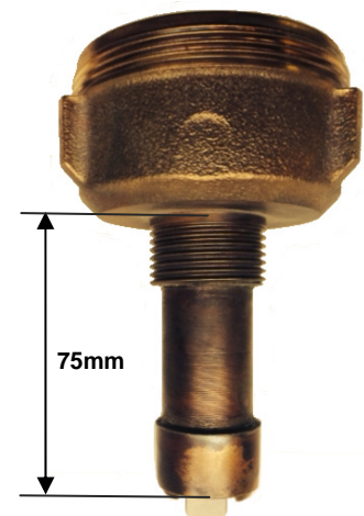
Long Stem body version for pipesizes > 150mm (other dimensions as at left)
